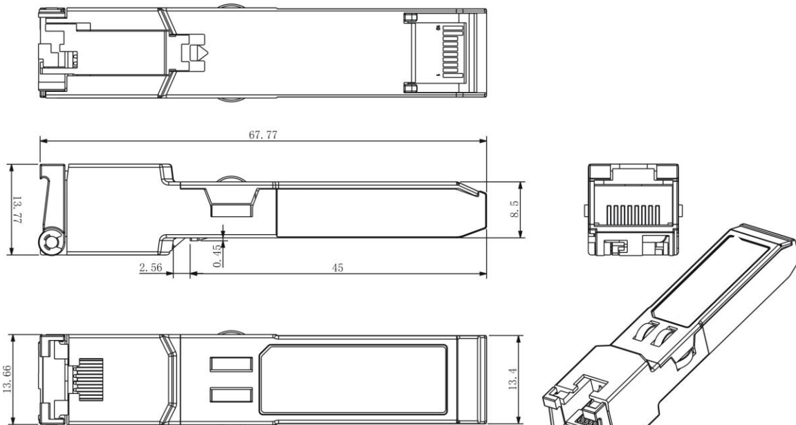
COPPER SFP Transceiver (Unit: mm View:
